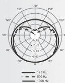
Polar Pattern
